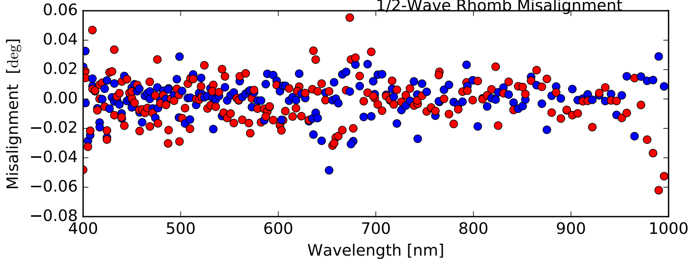
1/2-Wave Rhomb Misalignment
